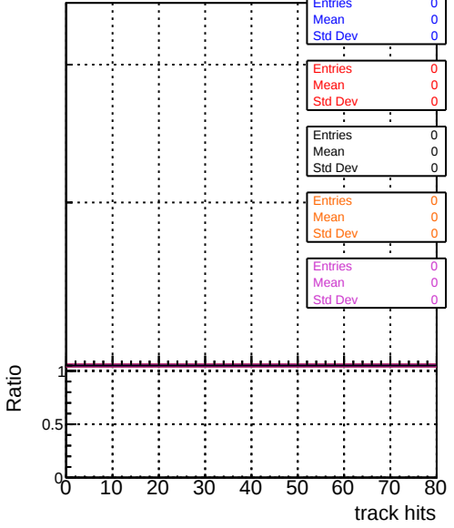
mean hit Legend: DOM mkFit XiMinusNOPU NEWdefault specPless1 DOM mkFit XiMinusNOPU NEWdefault specPless3 DOM mkFit XiMinusNOPU NEWdefault specPless4
