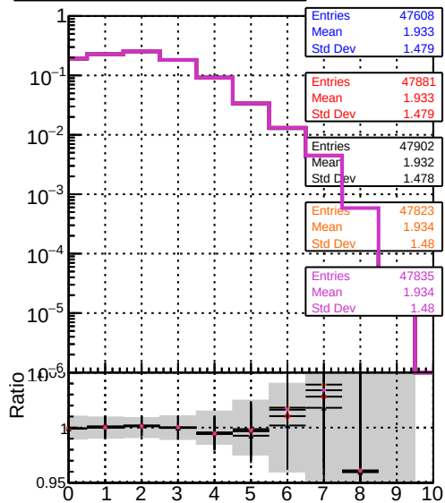
mean hits DOM mkFit XiMinusNOPU NEWdefault specPless1 DOM mkFit XiMinusNOPU NEWdefault specPless2 DOM mkFit XiMinusNOPU NEWdefault specPless3 DOM mkFit XiMinusNOPU NEWdefault specPless4
