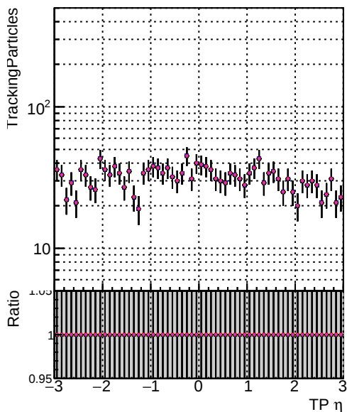
DOM mkFit XiMinusNOPU newDefault5 DOM mkFit XiMinusNOPU NEWdefault 5 DOM mkFit XiMinusNOPU NEWdefault 5 DOM mkFit XiMinusNOPU NEWdefault 5 DOM mkFit XiMinusNOPU NEWdefault 5
