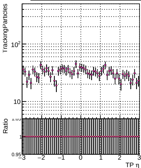
N of sin DOM mkFit XiMinus NOPU NEWdefault s DOM mkFit XiMinus NOPU NEWdefault s DOM mkFit XiMinus NOPU NEWdefault s
