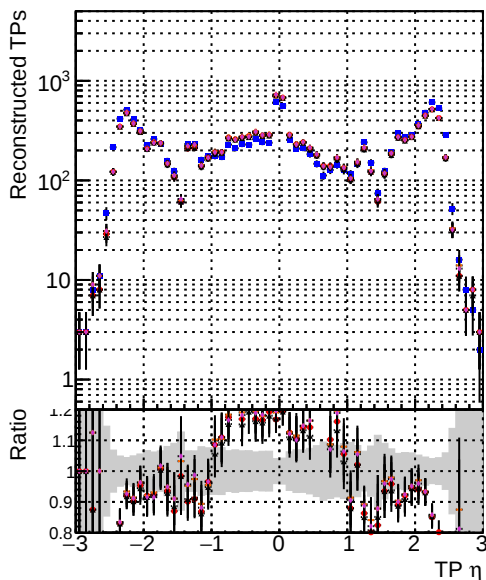
N of sim Model Method Model Method Model Method 1 DOM mkFit XiMinusNOPU NEWdefault specPless2 2 DOM mkFit XiMinusNOPU NEWdefault specPless3 3 DOM mkFit XiMinusNOPU NEWdefault specPless4
