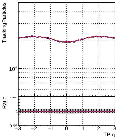
N of sim Model Method Model Method Model Method 1 DOM mkFit XiMinusNOPU NEWdefault specPless2 2 DOM mkFit XiMinusNOPU NEWdefault specPless3 3 DOM mkFit XiMinusNOPU NEWdefault specPless4
