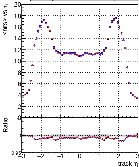
mean hits DOM mkFit TT NEWdefault specPless1 DOM mkFit TT NEWdefault specPless2 DOM mkFit TT NEWdefault specPless3 DOM mkFit TT NEWdefault specPless4
