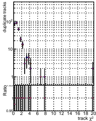
N of associated (recoSim) loopier tracks vs normalized \chi^2
