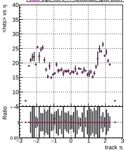
mean hit DOM mkFit TT NEWdefault specPless1 DOM mkFit TT NEWdefault specPless2 DOM mkFit TT NEWdefault specPless3 DOM mkFit TT NEWdefault specPless4
