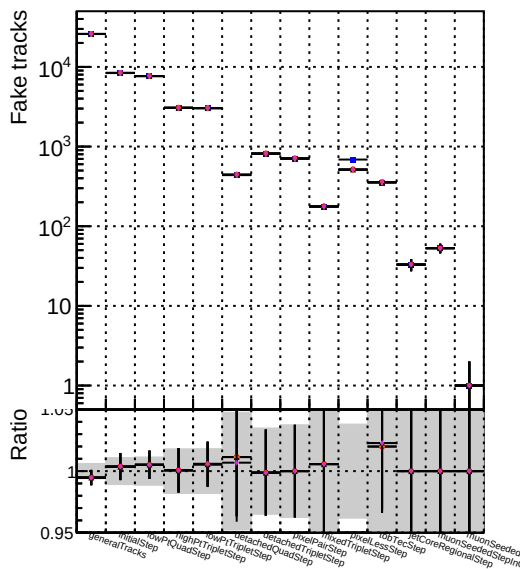
Number DOM mkFit TT NEWdefault specPless2 DOM mkFit TT NEWdefault specPless3 DOM mkFit TT NEWdefault specPless4
