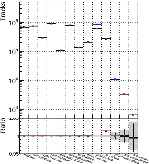
Number Model Method Dataset Spec PLess 1 DOM mkFit TT NEWdefault specPLess1 2 DOM mkFit TT NEWdefault specPLess2 3 DOM mkFit TT NEWdefault specPLess3 4 DOM mkFit TT NEWdefault specPLess4
