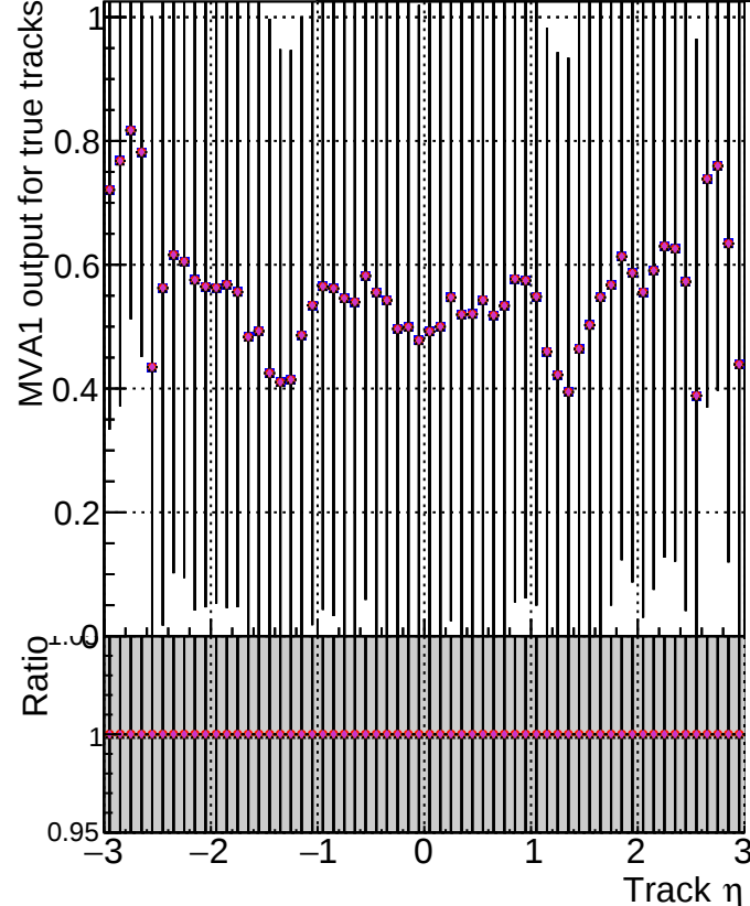
MVA1 of associated tracks (recoToSim) vs. track \eta Legend: DOM mkFit TT retrain DOM mkFit TT NEWdefault specPless1 DOM mkFit TT NEWdefault specPless2 DOM mkFit TT NEWdefault specPless3 DOM mkFit TT NEWdefault specPless4
