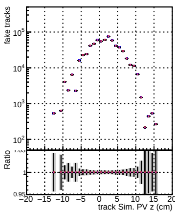
N of fake tracks vs. sim PV z
