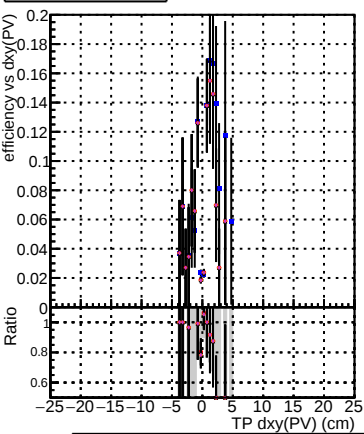
Efficiency vs Dxy(PV) Legend: DOM_mkFit_TT_retrain DOM_mkFit_TT_NEWdefault_specPless1 DOM_mkFit_TT_NEWdefault_specPless2 DOM_mkFit_TT_NEWdefault_specPless3 DOM_mkFit_TT_NEWdefault_specPless4
