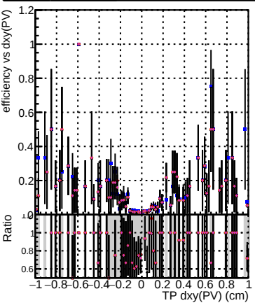
Efficiency vs Dxy(PV) Legend: DOM_mkFit_TT_retrain DOM_mkFit_TT_NEWdefault_specPless1 DOM_mkFit_TT_NEWdefault_specPless2 DOM_mkFit_TT_NEWdefault_specPless3 DOM_mkFit_TT_NEWdefault_specPless4
