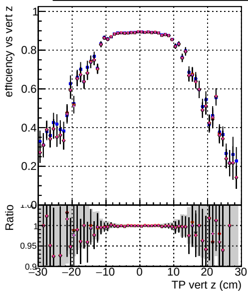
Efficiend DOM mkFit TT NEWdefault specPless2 DOM mkFit TT NEWdefault specPless3 DOM mkFit TT NEWdefault specPless4
