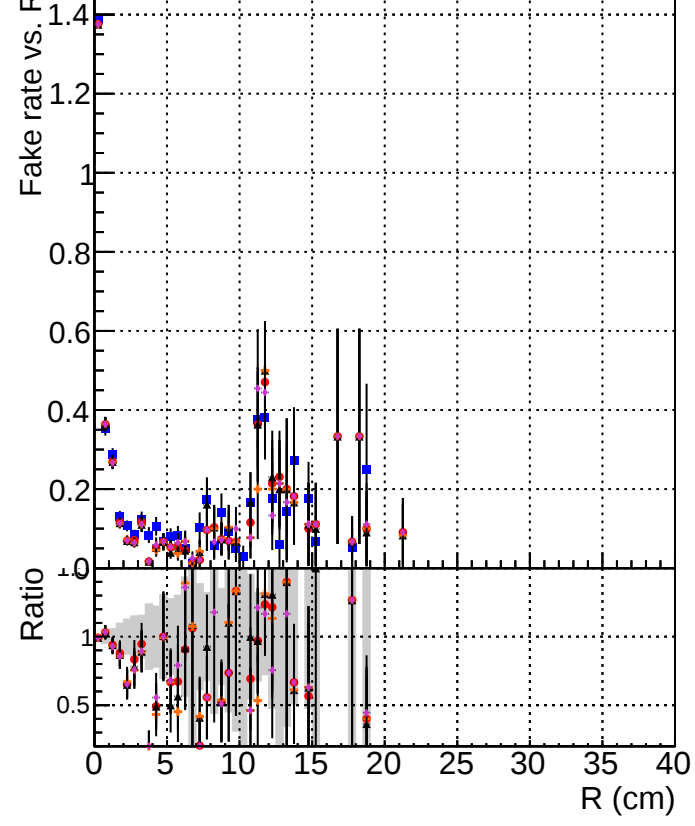
K_S^0 tracking fake rate vs R DOM_mkFit_TT_retrain DOM_mkFit_TT_NEWdefault_specPLess1 DOM_mkFit_TT_NEWdefault_specPLess2 DOM_mkFit_TT_NEWdefault_specPLess3 DOM_mkFit_TT_NEWdefault_specPLess4
