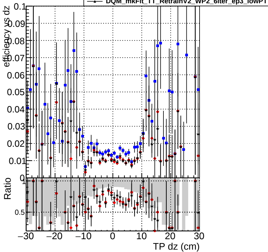
Efficiency vs Dz
