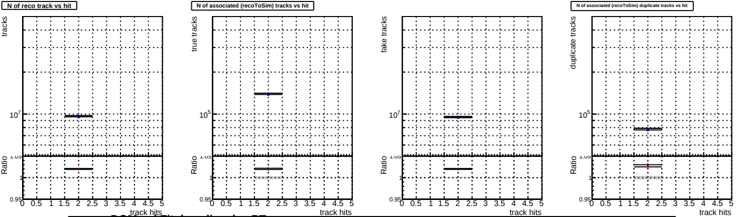
N of reco track vs hit N of associated (recoToSim) tracks vs hit fake tracks N of associated (recoToSim) duplicate tracks vs hit DQM_mkFit_baseline_lowPT DQM_mkFit_baseline6iter_lowPT DQM_mkFit_TT_RetrainV2_WP2_6iter_ep3_lowPT
