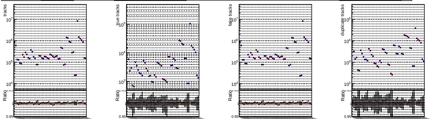
N of reco track vs. \chi^2
