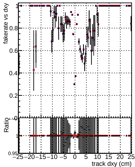
DOM mkFit baseline lowPT DOM mkFit baselineGiter lowPT Fake rate vs d — DOM mkFit 11 Retrain v2 WP2 6iter ep3 lowPT
