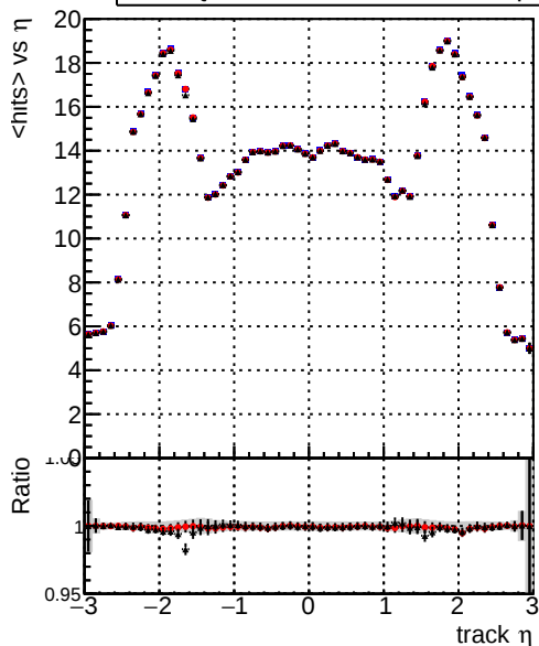
mean hits vs \eta Legend: - DQM_mkFit_baseline_lowPT (blue line) - DQM_mkFit_baseline6iter_lowPT (red line) - DQM_mkFit_TT_RetrainV2_WP2_6iter_ep3_lowPT (black line)
