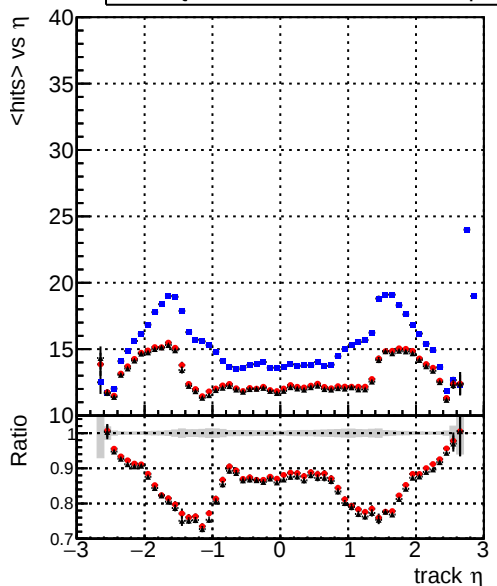
mean hits vs \eta — DQM_mkFit_baseline_lowPT — DQM_mkFit_baseline6iter_lowPT — DQM_mkFit_TT_RetrainV2_WP2_6iter_ep3_lowPT
