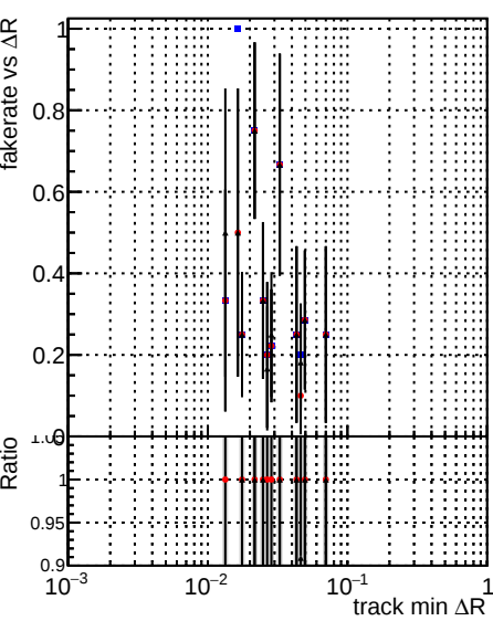
Legend: DQM_mkFit_baseline_lowPT (blue), DQM_mkFit_baseline6iter_lowPT (red), DQM_mkFit_TT_RetrainV2_WP2_6iter_ep3_lowPT (black)
