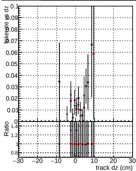
— DOM mkFit baseline lowPT — DOM mkFit baselineGiter lowPT — DOM mkFit TT Retrain2 WP2 6iter ep3 lowPT
