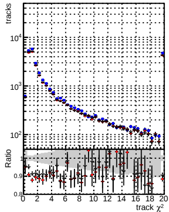
N of reco track vs. \chi^2 for baseline lowPT, Retrain V2, WP2, 6iter, ep3 lowPT
