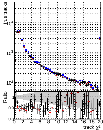
N of reco track vs. \chi^2 for baseline lowPT, Retrain V2, WP2, 6iter, ep3 lowPT
