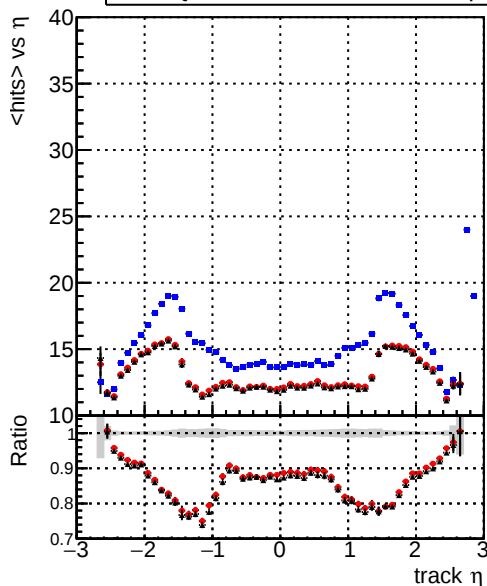
mean hits vs \eta — DQM_mkFit_baseline_lowPT — DQM_mkFit_baseline6iter_lowPT — DQM_mkFit_TT_RetrainV2_WP2_6iter_ep3_lowPT
