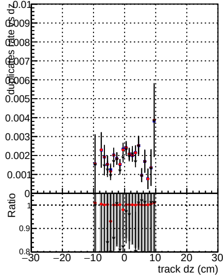
— DOM mkFit baseline lowPT — DOM mkFit baseline giter lowPT — DOM mkFit Retrain v2 WP2 giter ep3 lowPT
