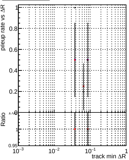
Legend: DQM_mkFit_baseline_lowPT (blue dots), DQM_mkFit_baseline6iter_lowPT (red dots), DQM_mkFit_TT_RetrainV2_WP2_6iter_ep3_lowPT (black dots)
