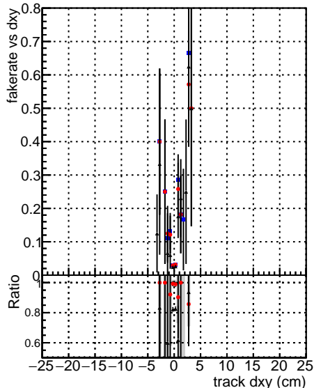
—●— DGM mkFit baseline lowPT —●— DGM mkFit baseline Giter lowPT —●— DGM mkFit 1T RetrainV2 WP2 Giter ep3 lowPT
