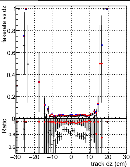
—●— DGM mkFit baseline lowPT —●— DGM mkFit baseline Giter lowPT —●— DGM mkFit 1T RetrainV2 WP2 Giter ep3 lowPT
