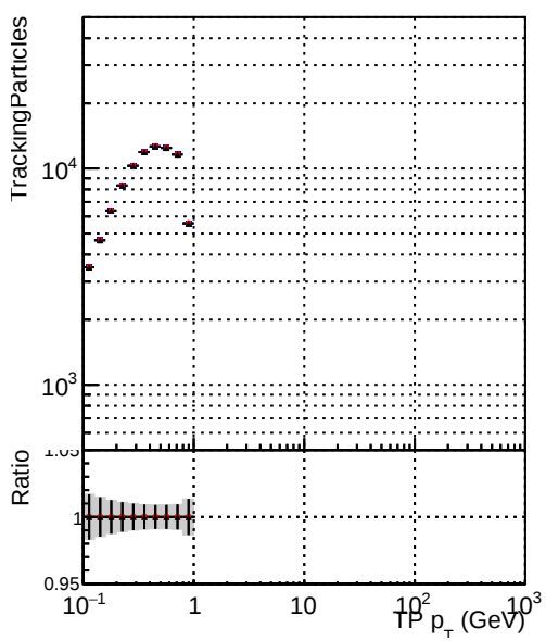
Legend: - DQM_mkFit_baseline_lowPT (blue line with dots) - DQM_mkFit_baseline6iter_lowPT (red line with dots) - DQM_mkFit_TT_RetrainV2_WP2_6iter_ep3_lowPT (black line with dots)
