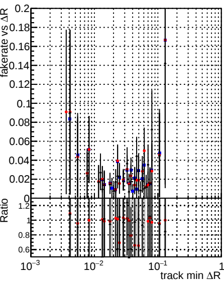
Fake rate vs \Delta R(\text{track, jet}) Legend: DQM_mkFit_baseline_lowPT DQM_mkFit_baseline6iter_lowPT DQM_mkFit_TT_RetrainV2_WP2_6iter_ep3_lowPT
