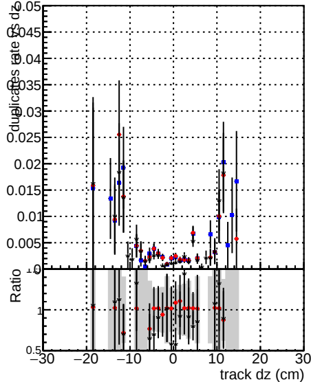
— DOM mkFit baseline lowPT — DOM mkFit baseline 6iter lowPT — DOM mkFit 11 Retrain v2 WP2 — DOM mkFit 6iter ep3 lowPT
