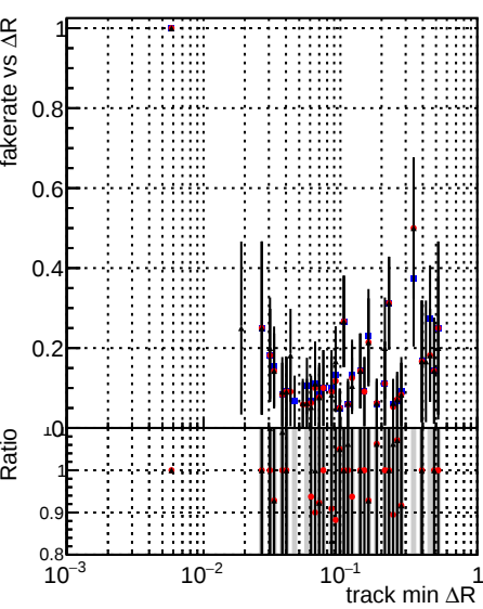
Legend: DQM_mkFit_baseline_lowPT (black), DQM_mkFit_baseline6iter_lowPT (red), DQM_mkFit_TT_RetrainV2_WP2_6iter_ep3_lowPT (blue)
