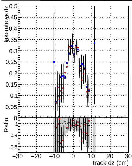
Fake rate vs dz Legend: DOM mkFit baseline lowPT (blue squares) DOM mkFit baseline giter lowPT (red circles) DOM mkFit TT Retrain v2 WP2 (black circles)
