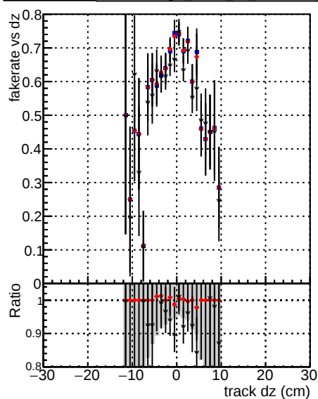
Fake rate vs dz Legend: DOM mkFit baseline lowPT DOM mkFit baseline giter lowPT DOM mkFit TT Retrain v2 WP2
