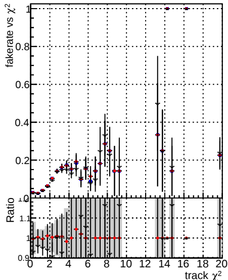
Fake rate vs. \chi^2 Legend: DOM mkFit baseline lowPT DOM mkFit baseline 6iter lowPT DOM mkFit TT Retrain v2 WP2 6iter ep3 lowPT
