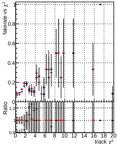
Fake rate vs. 6iter ep3 lowPT
