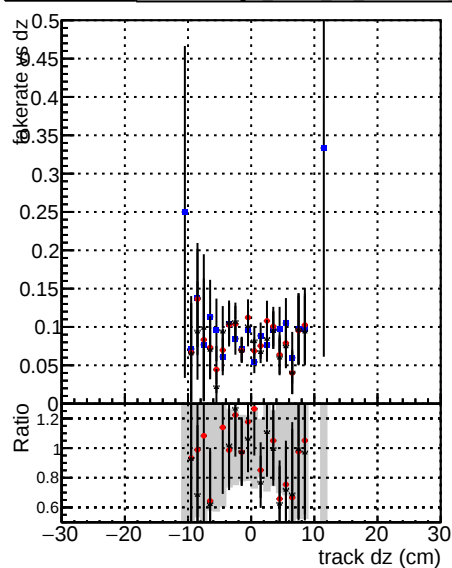
DOM mkFit baseline lowPT DOM mkFit baseline giter lowPT DOM mkFit TT Retrain v2 WP2 giter ep3 lowPT
