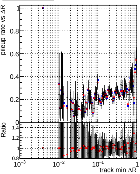
Legend: DQM_mkFit_baseline_lowPT (blue circles), DQM_mkFit_baseline6iter_lowPT (red circles), DQM_mkFit_TT_RetrainV2_WP2_6iter_ep3_lowPT (black circles)
