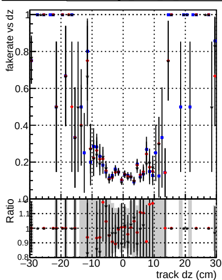
DOM mkFit baseline lowPT DOM mkFit baseline giter lowPT DOM mkFit TT Retrain v2 WP2
