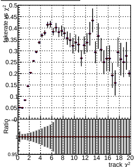
Fake rate vs. \chi^2 for 6iter ep3 lowPT
