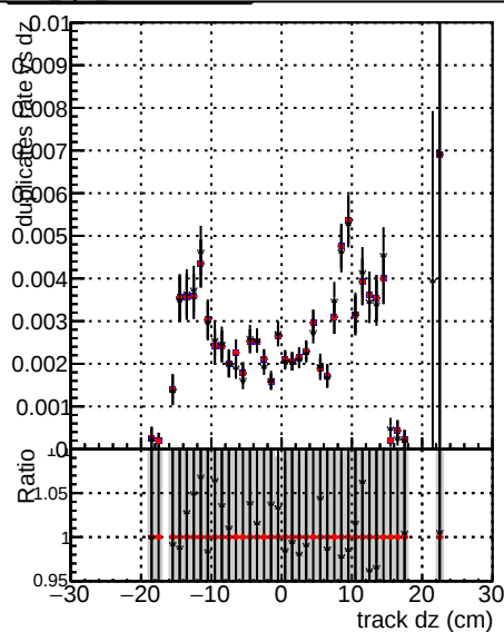
— DOM mkFit baseline lowPT — DOM mkFit baseline giter lowPT — DOM mkFit TT Retrain/2 WP2 giter ep3 lowPT
