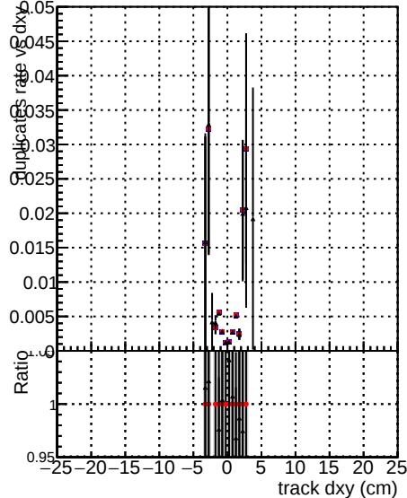
— DOM mkFit baseline lowPT — DOM mkFit baseline giter lowPT — DOM mkFit TT Retrain/2 WP2 giter ep3 lowPT
