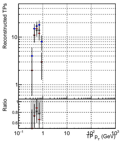
Legend: DQM_mkFit_baseline_lowPT (blue dots), DQM_mkFit_baseline6iter_lowPT (red dots), DQM_mkFit_TT_RetrainV2_WP2_6iter_ep3_lowPT (black dots with error bars)
