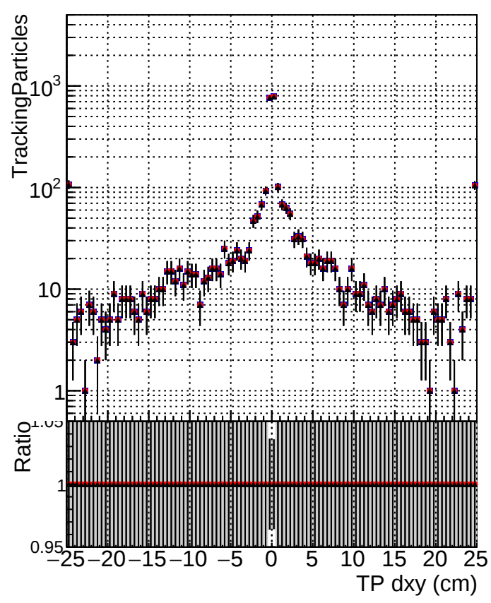
N of simulated track ■ DQM_mkFit_baseline_lowPT ● DQM_mkFit_baseline6iter_lowPT ▲ DQM_mkFit_TT_RetrainV2_WP2_6iter_ep3_lowPT
