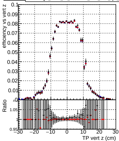
Efficiency vs. sim PV z — DQM_mkFit_baseline_lowPT — DQM_mkFit_baseline6iter_lowPT — DQM_mkFit_TT_RetrainV2_WP2_6iter_ep3_lowPT
