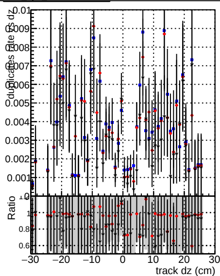
— DOM mkFit baseline lowPT — DOM mkFit baseline giter lowPT — DOM mkFit 11 Retrain v2 WP2 giter ep3 lowPT
