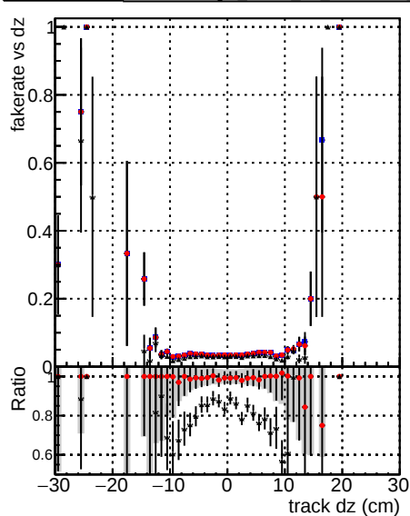
DOM mkFit baseline lowPT DOM mkFit baseline 6iter lowPT DOM mkFit TT Retrain v2 WP2 6iter ep3 lowPT
