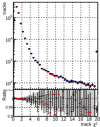
DOM mklFit baseline lowPT DOM mklFit baseline6iter lowPT DOM mklFit 11 RetrainV2 WP2 6iter ep3 lowPT
