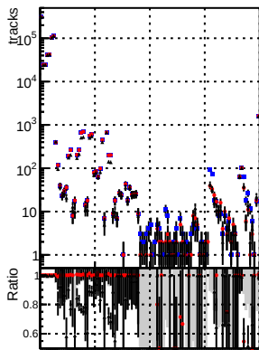
DOM mklFit baseline lowPT DOM mklFit baseline6iter lowPT DOM mklFit 11 RetrainV2 WP2 6iter ep3 lowPT
