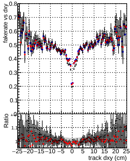
DOM mkFit baseline lowPT DOM mkFit baselineGiter lowPT DOM mkFit 11 Retrain2 WP1 6iter ep3 lowPT
