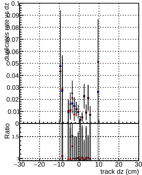
DOM mkFit baseline lowPT DOM mkFit baseline 6iter lowPT DOM mkFit Retrain v2 WP1
