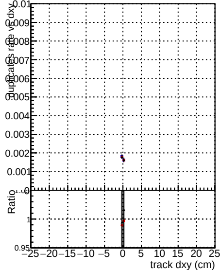
DOM mkFit baseline lowPT DOM mkFit baseline 6iter lowPT DOM mkFit 11 Retrain v2 WP1 6iter ep3 lowPT
